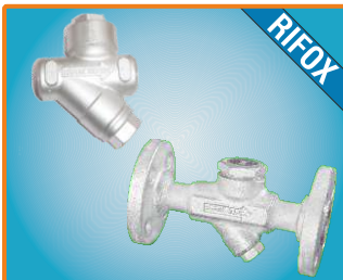
THERMODYNAMIC STEAM TRAP
